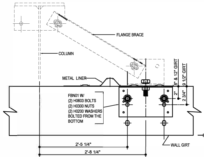
TYPICAL FLANGE BRACE@ GIRT & COLUMN W/ LINER
