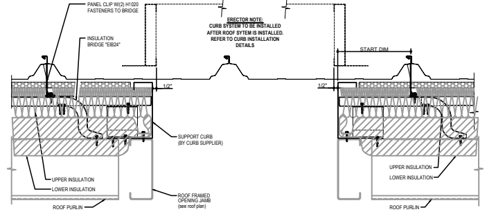
SEC 'B'-'B' SUPPORT CURB & BRIDGE TERMINATION
