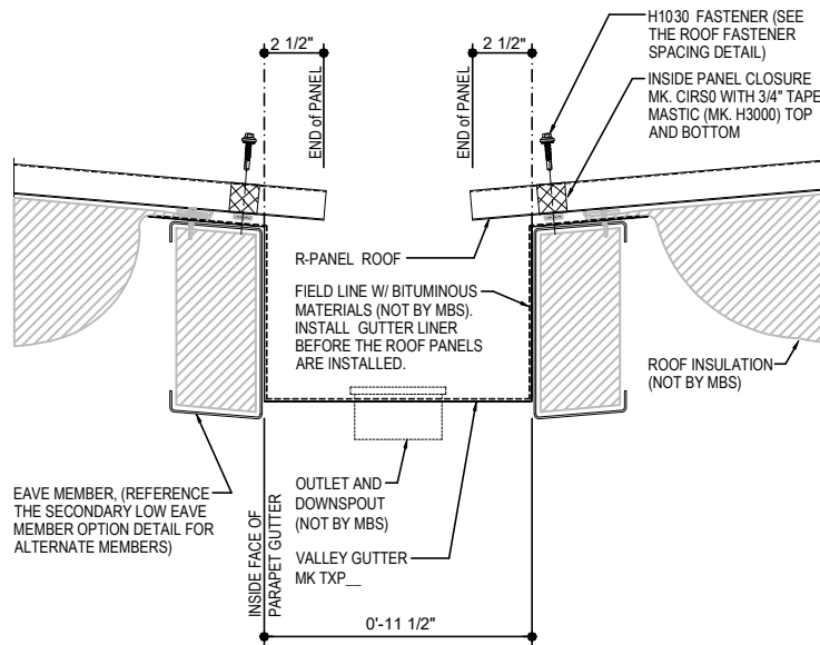
VALLEY GUTTER INSTALLATION R-Panel LOW EAVE DETAIL w/ VALLEY GUTTER
