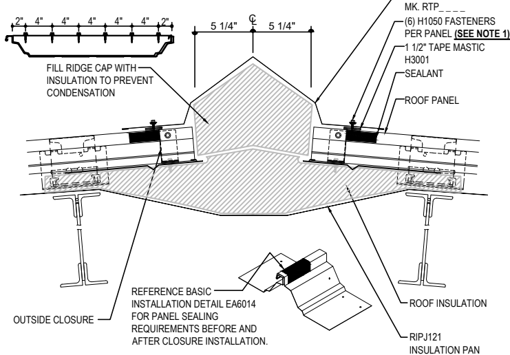
RIDGE TRIM DETAIL RIDGE TRIM DETAIL
