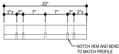
FLASHING ENDLAP BACKER FIELD CUT FROM STANDARD FEB120
