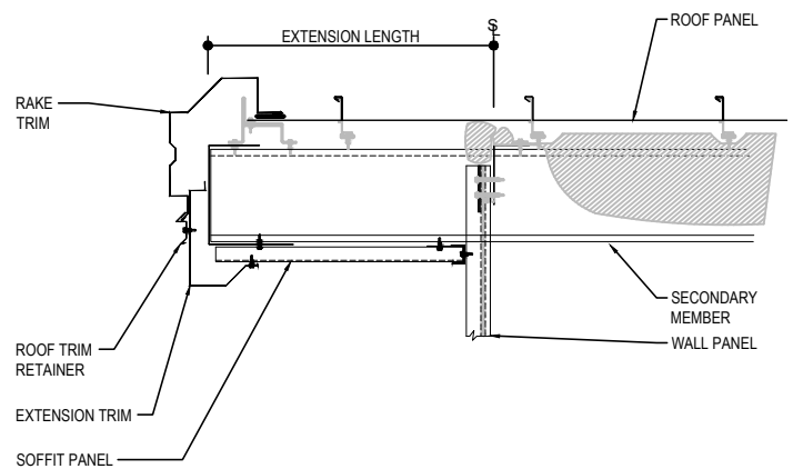
RAKE EXTENSION - IMP WALL w / FLAT SL PANEL SOFFIT
