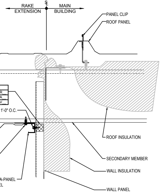
RAKE EXTENSION SOFFIT AT BUILDING STEEL LINE
