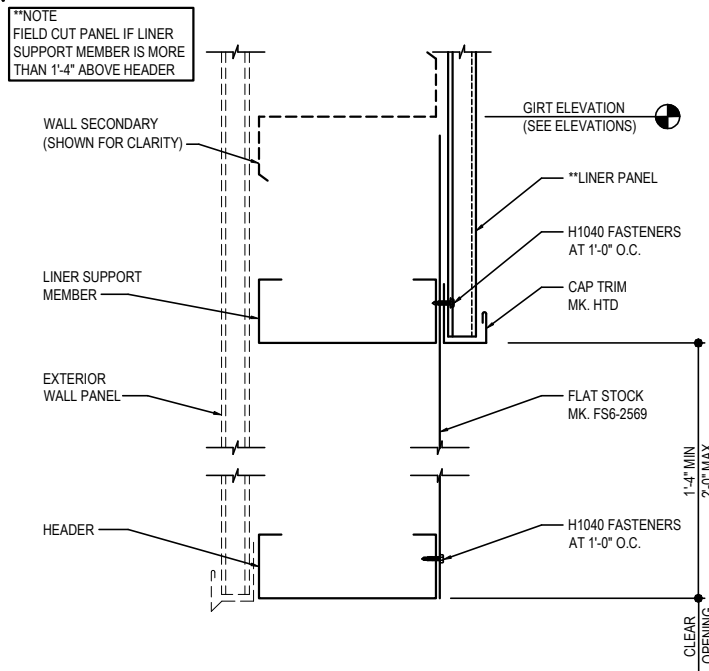
SECONDARY > 2'-0" ABOVE HEADER
