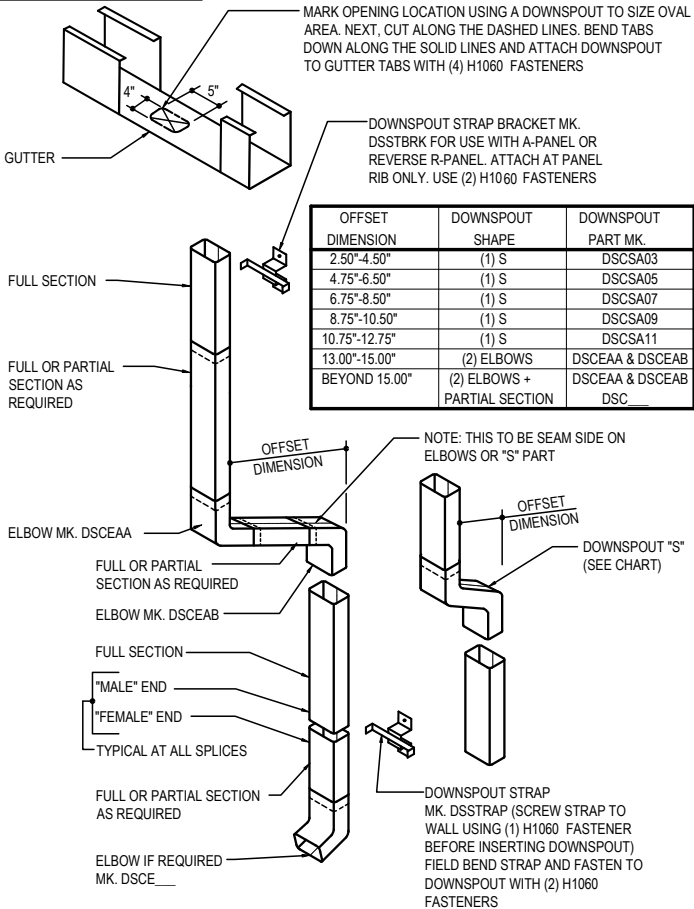
CORRUGATED DOWNSPOUT AT INSET WALL REFERENCE GUTTER AND DOWNSPOUT SCHEDULE FOR DOWNSPOUT MARK NUMBERS
