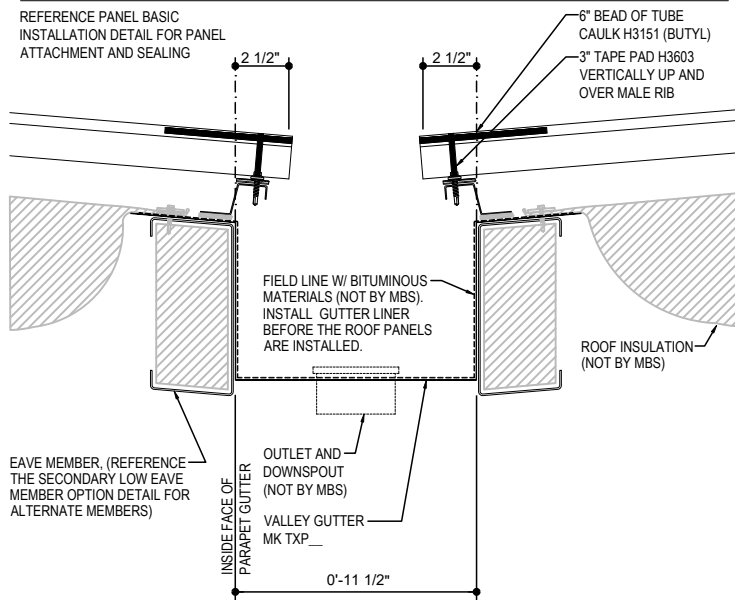
VALLEY GUTTER INSTALLATION LOW EAVE DETAIL W/ VALLEY GUTTER
